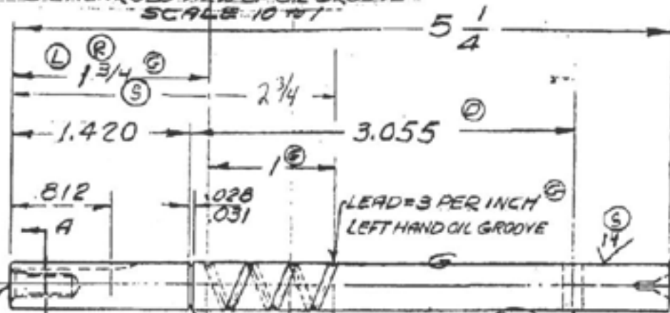
ENLARGED VIEW OF OIL GROOVE SCALE - 10:1
